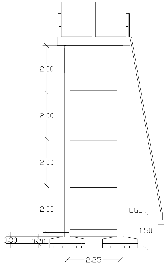
DETAILS OF MEMBERS & SCHEDULE OF REINFORCEMENT
