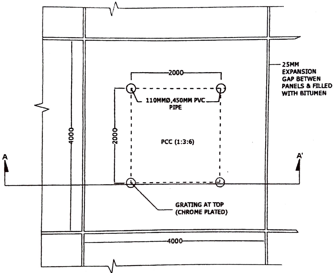
Fig.1: PLAN
