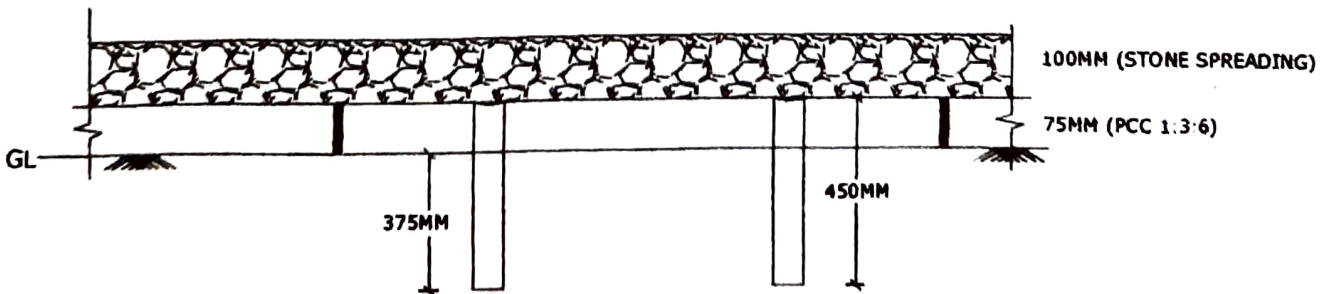
Fig.2: SECTION AA'
