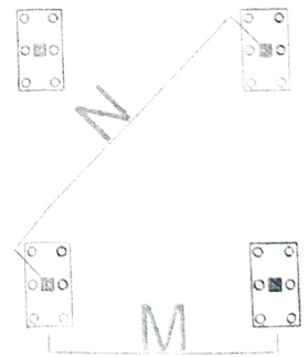
TRANSVERSE FACE PILE CAP PLAN FOR EACH TOWER LEG
