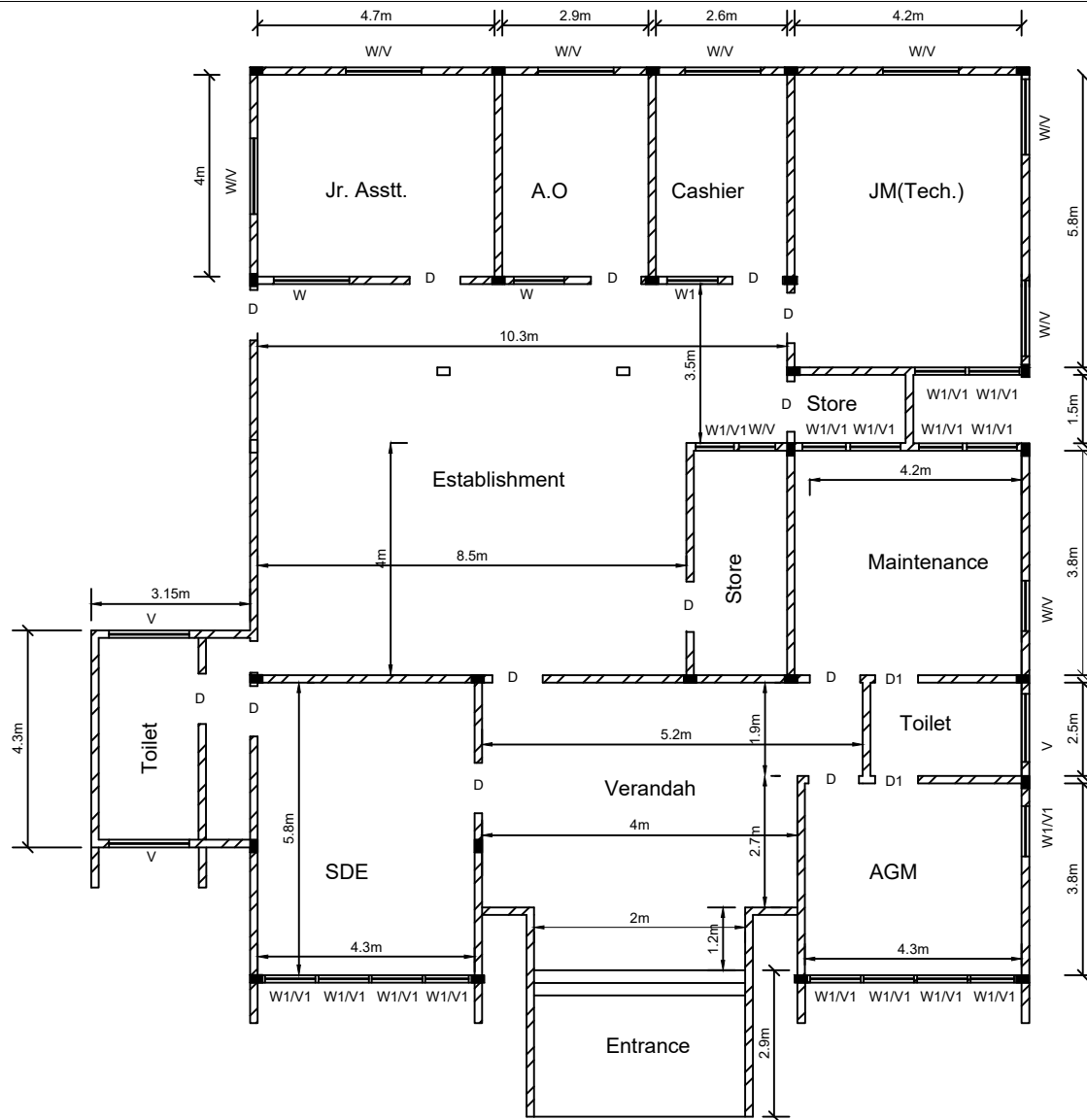
Fig.: Layout of Division Office, 220kV GSS, AEGCL, Mariani
