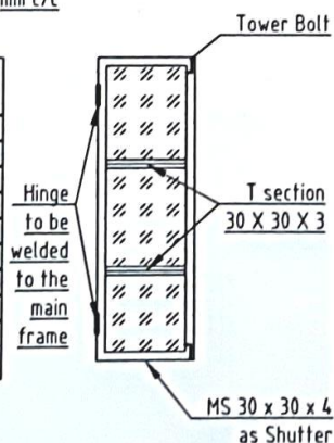
Single Shutter
