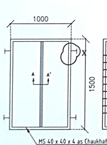
Window Frame
