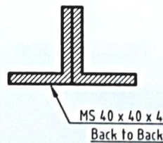
Enlarged Section A - A' details
