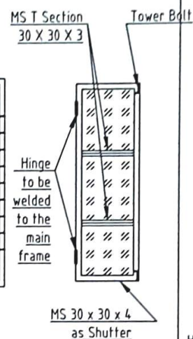
Single Shutter
