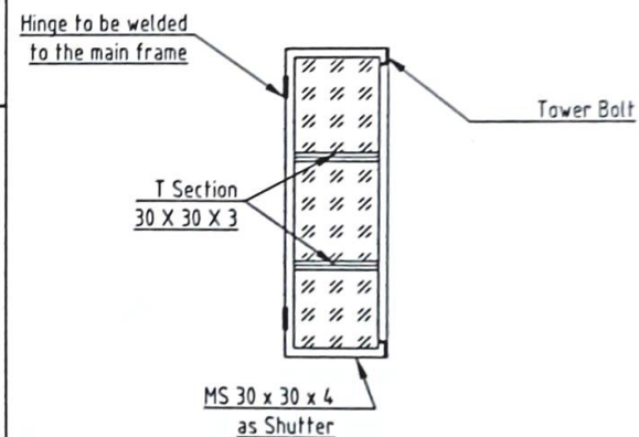
Single Shutter
