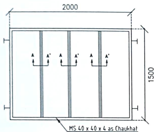
Window Frame
