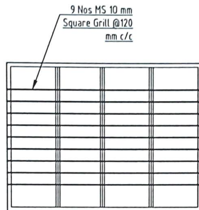
Window frame with Grill
