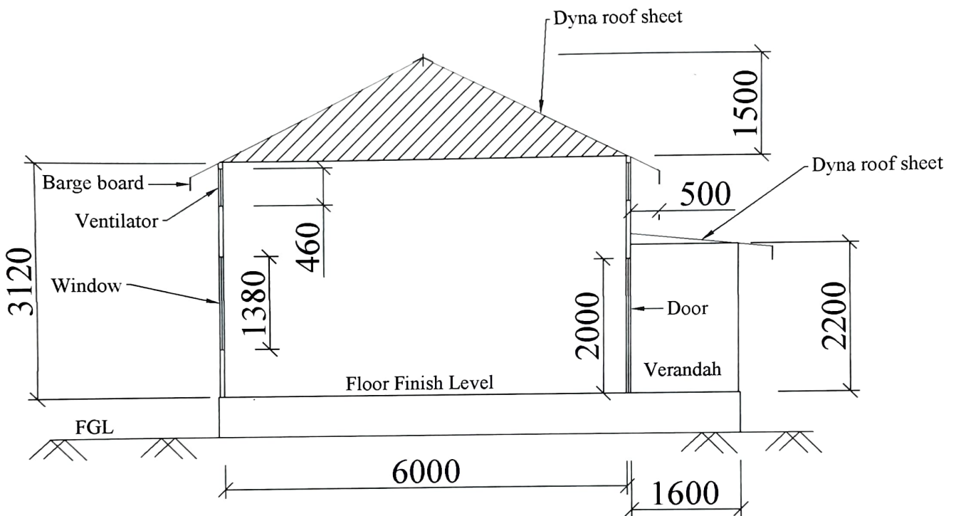
Side Elevation Section A-A'
