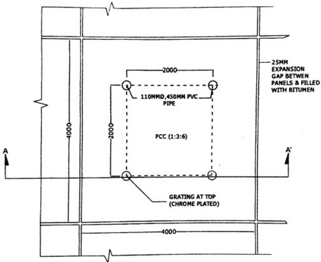
Fig.1: PLAN
