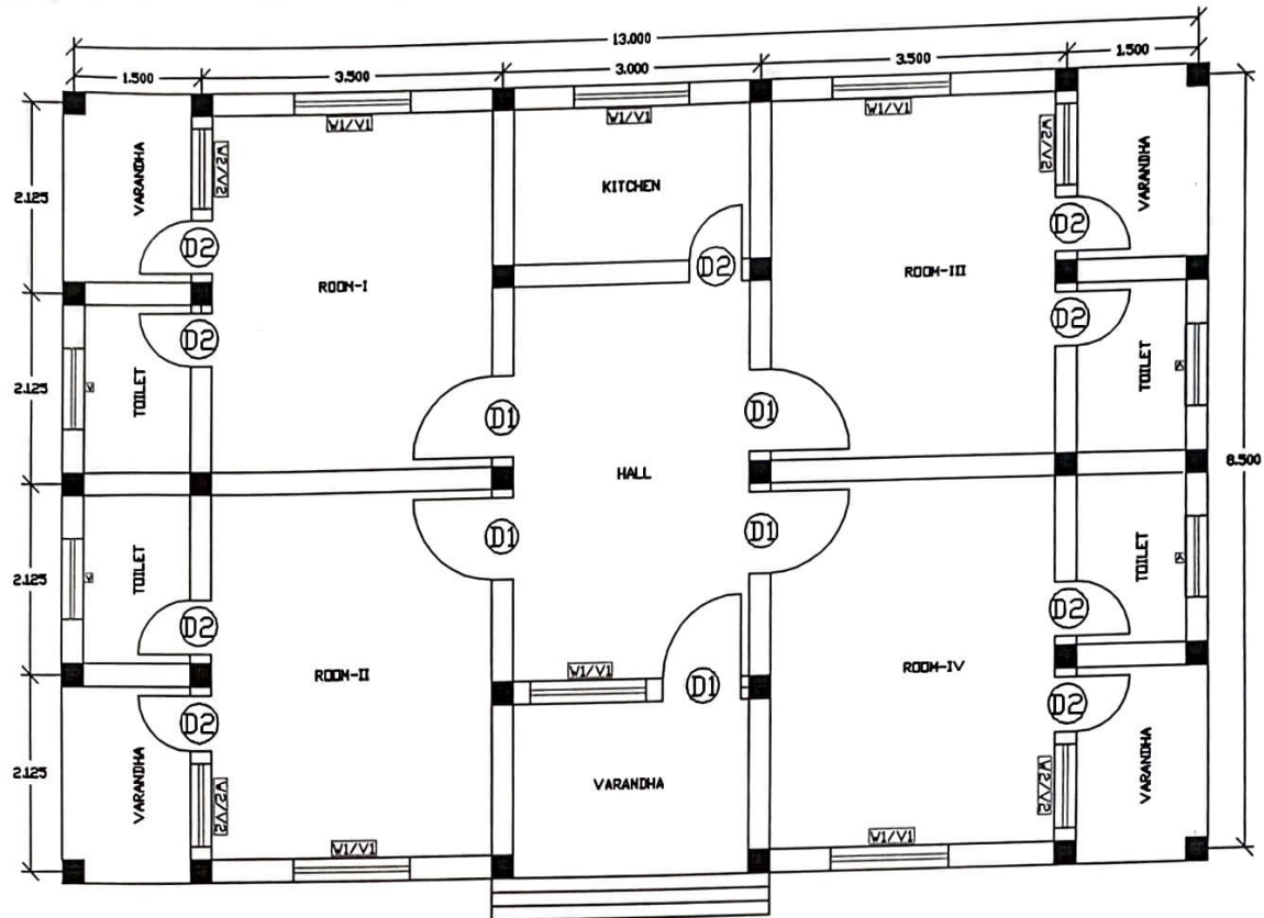
LAYOUT PLAN OF STAFF HOSTEL AT 132KV HAILAKANDI GSS
