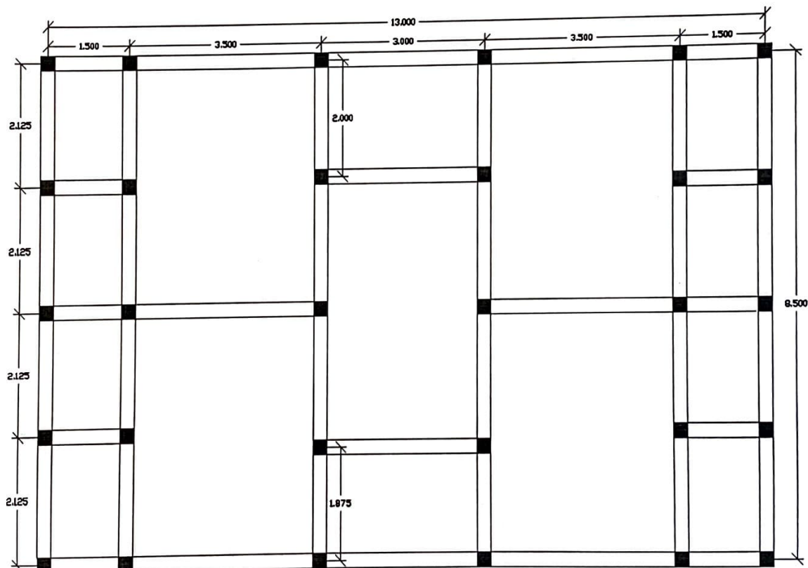
BEAM COLUMN LAYOUT OF STAFF HOSTEL AT 132KV HAILAKANDI GSS
