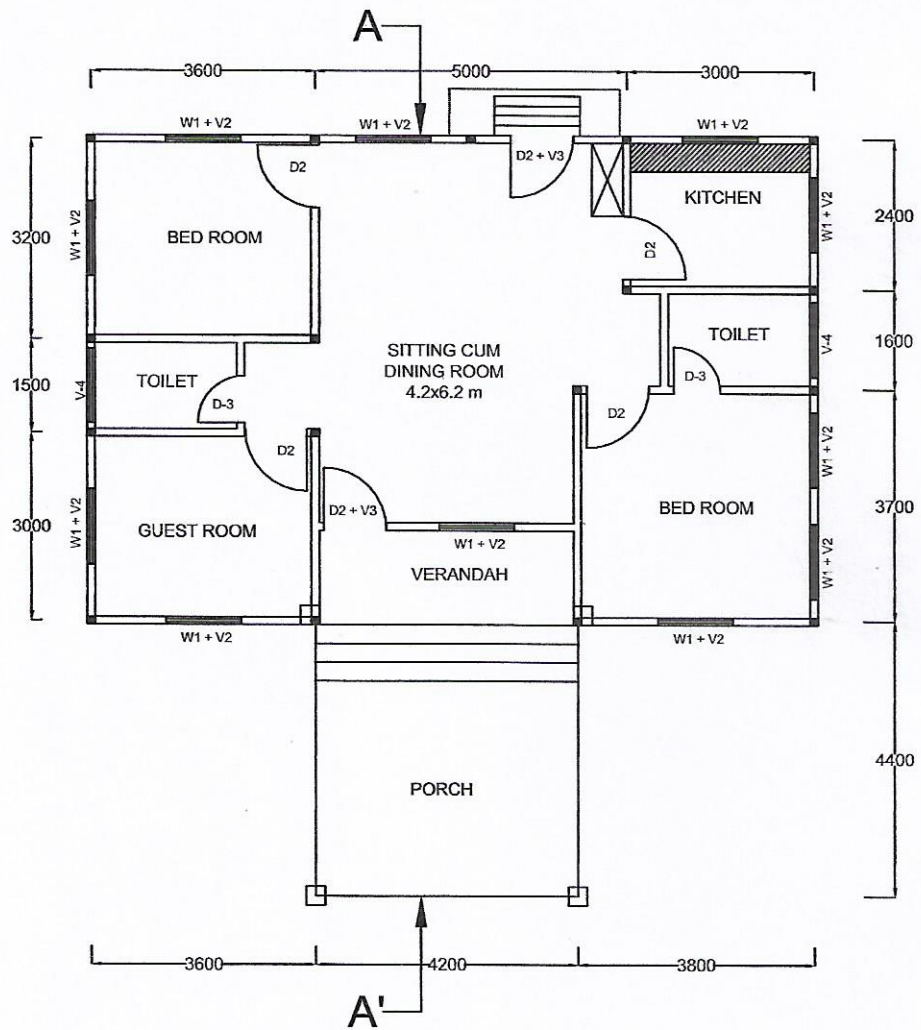
BUILDING LAYOUT
