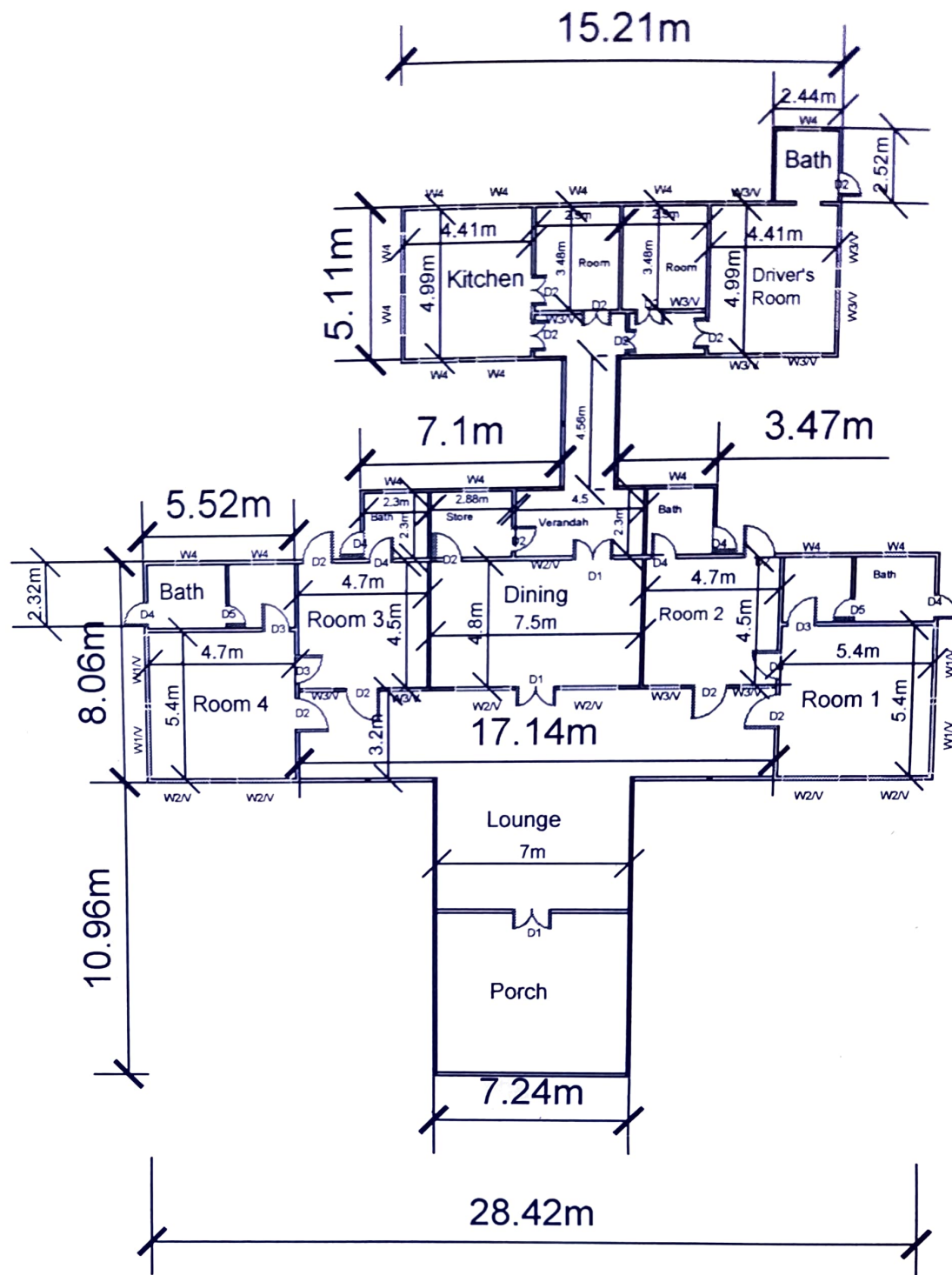
Layout of Guest House at 220kV GSS, AEGCL, Mariani
