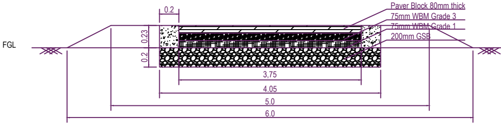
Fig: TYPICAL CROSS SECTION OF PAVER ROAD (3.75m width)
