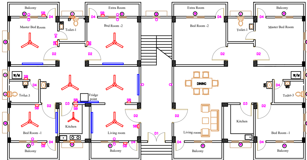
TOP VIEW/ PLAN OF THE PROPOSED G+2 RCC QUARTER
