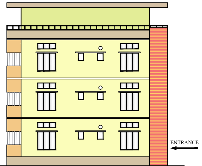
SIDE ELEVATION OF THE PROPOSED G+2 RCC QUARTER
