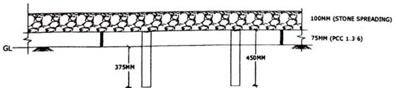
Fig.2: SECTION AA'
