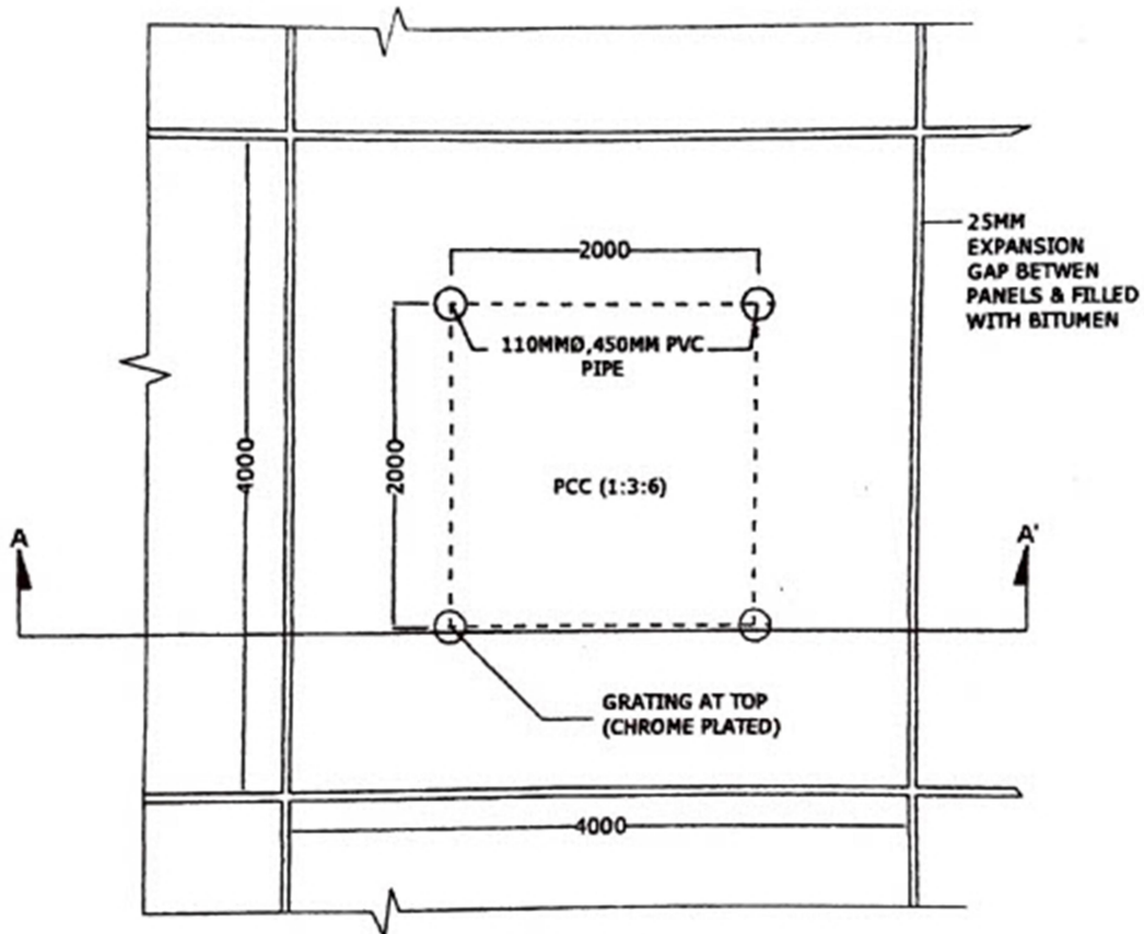
Fig.1: PLAN
