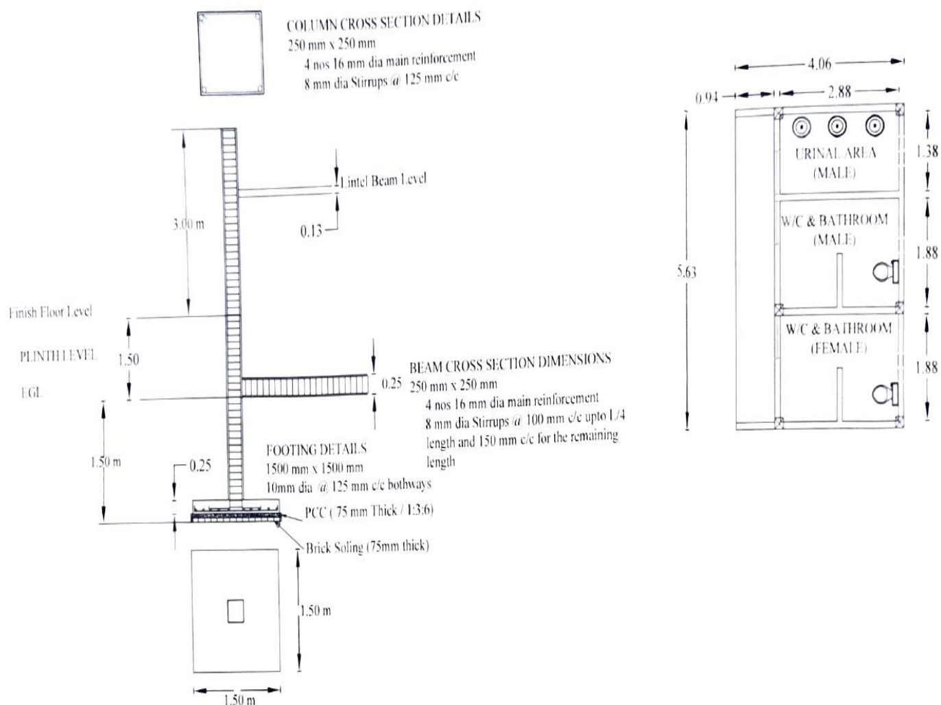
LAYOUT AND FOOTING DETAILS FOR CONSTRUCTION OF A NEW TOILET FOR THE CRB AT 220 KV GSS, AEGCL, SALAKATI.
